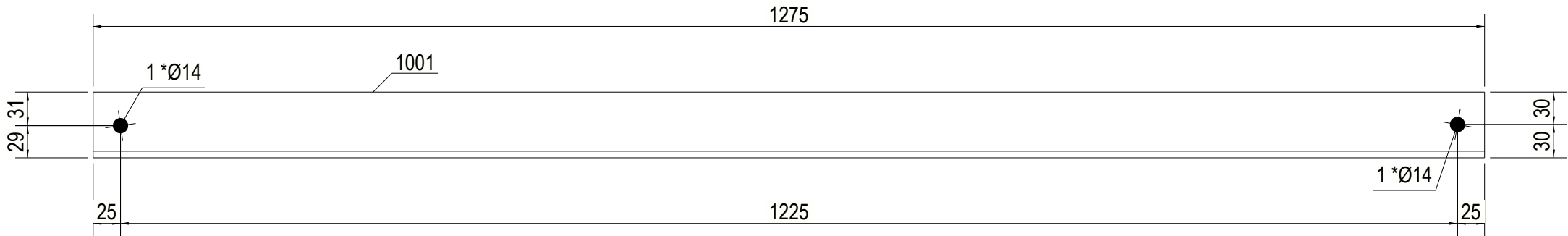
FRONT VIEW
